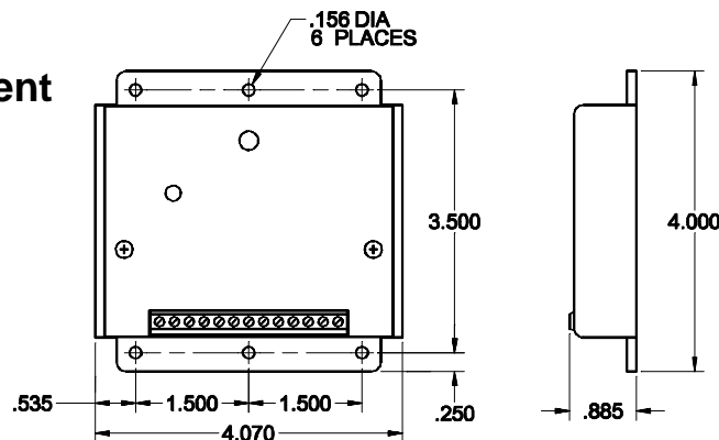
FIGURE 1: MBL536 DIMENSIONS
