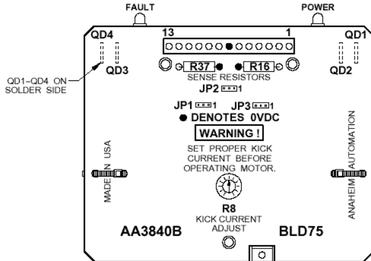
Figure 4: Jumper Location Drawing
