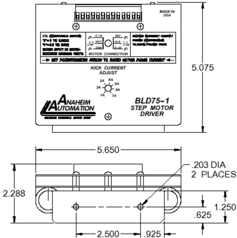
Figure 10: BLD75-1 Dimensions
