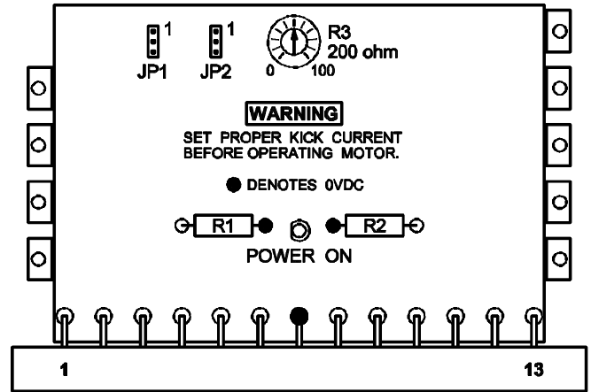
FIGURE 2: JUMPER LOCATIONS
