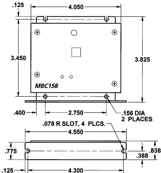
MBC158 Dimensions
